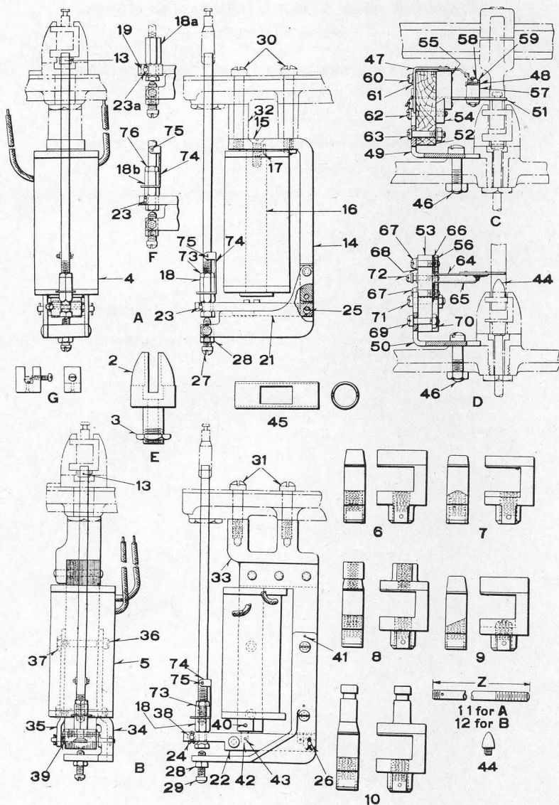
A. C. AND D. C. INDICATION MAGNETS, LATCHES AND LEVER LOCK CIRCUIT CONTROLLERS
